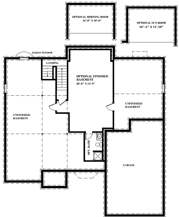
Foundation Plan
