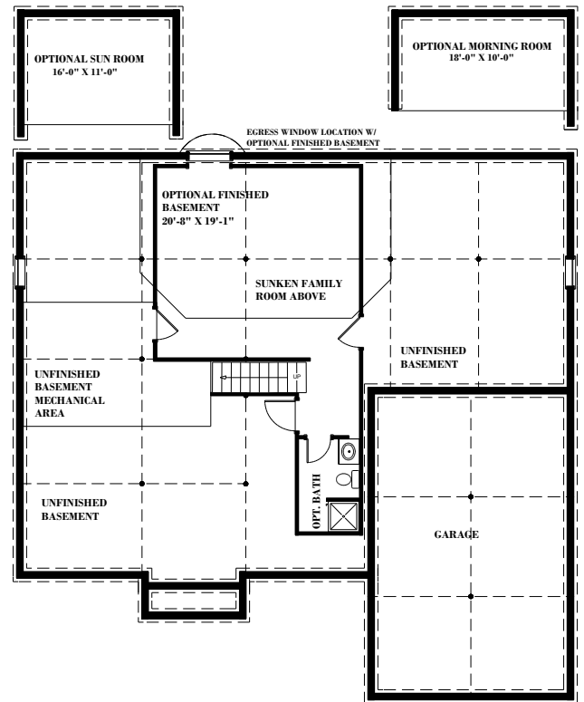
Foundation Plan
