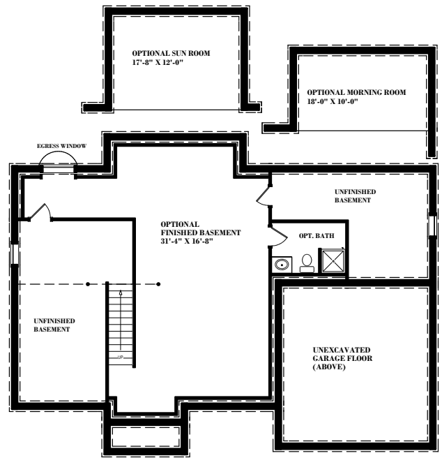
Foundation Plan
